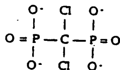
Clodronate
